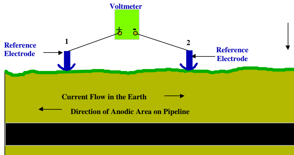
Figure 10 Positive Reading for Cell-To-Cell Survey
