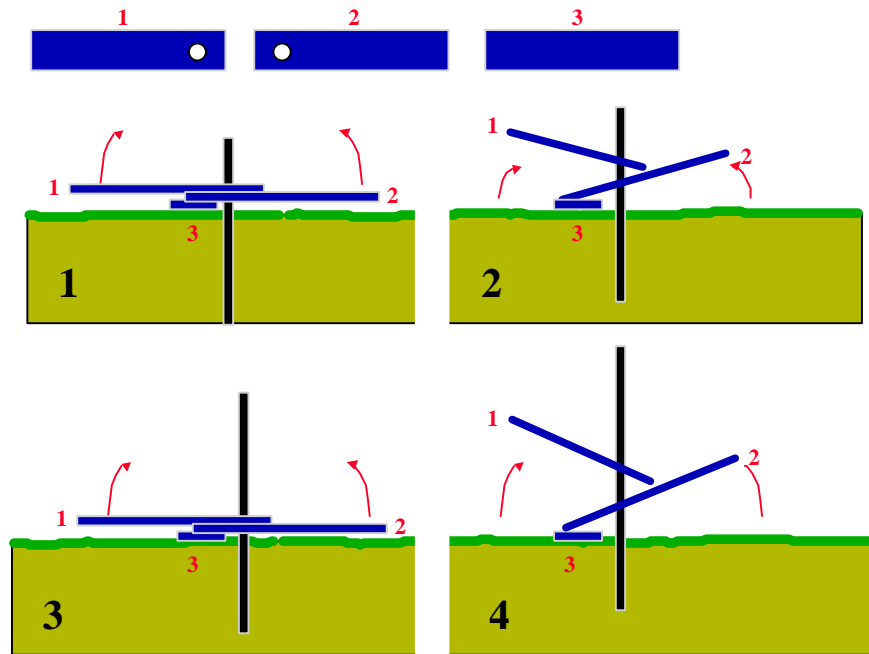
Figure 25 Removing Temporary Anodes (Ground Rods)
