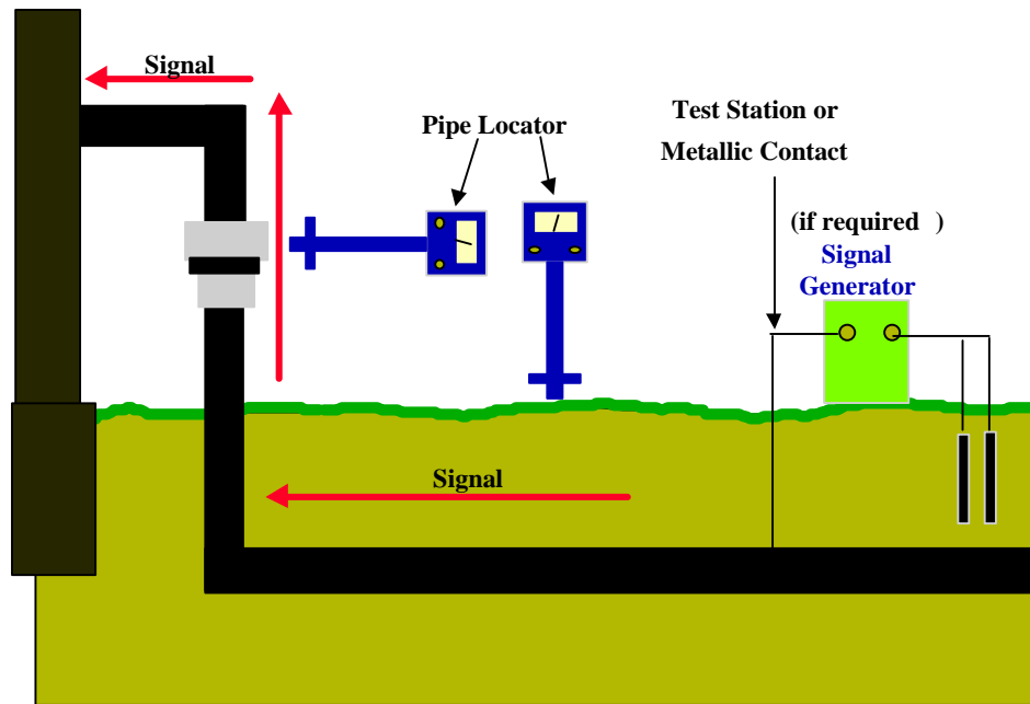
Figure 15 Testing for a Shorted Dielectric Using a Pipe Locator
