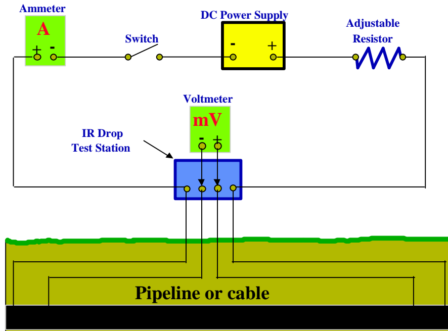
Figure 34 Calibration of an IR Drop Test Span
